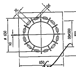
UPPER PLATE DETAIL SCALE NTS.
