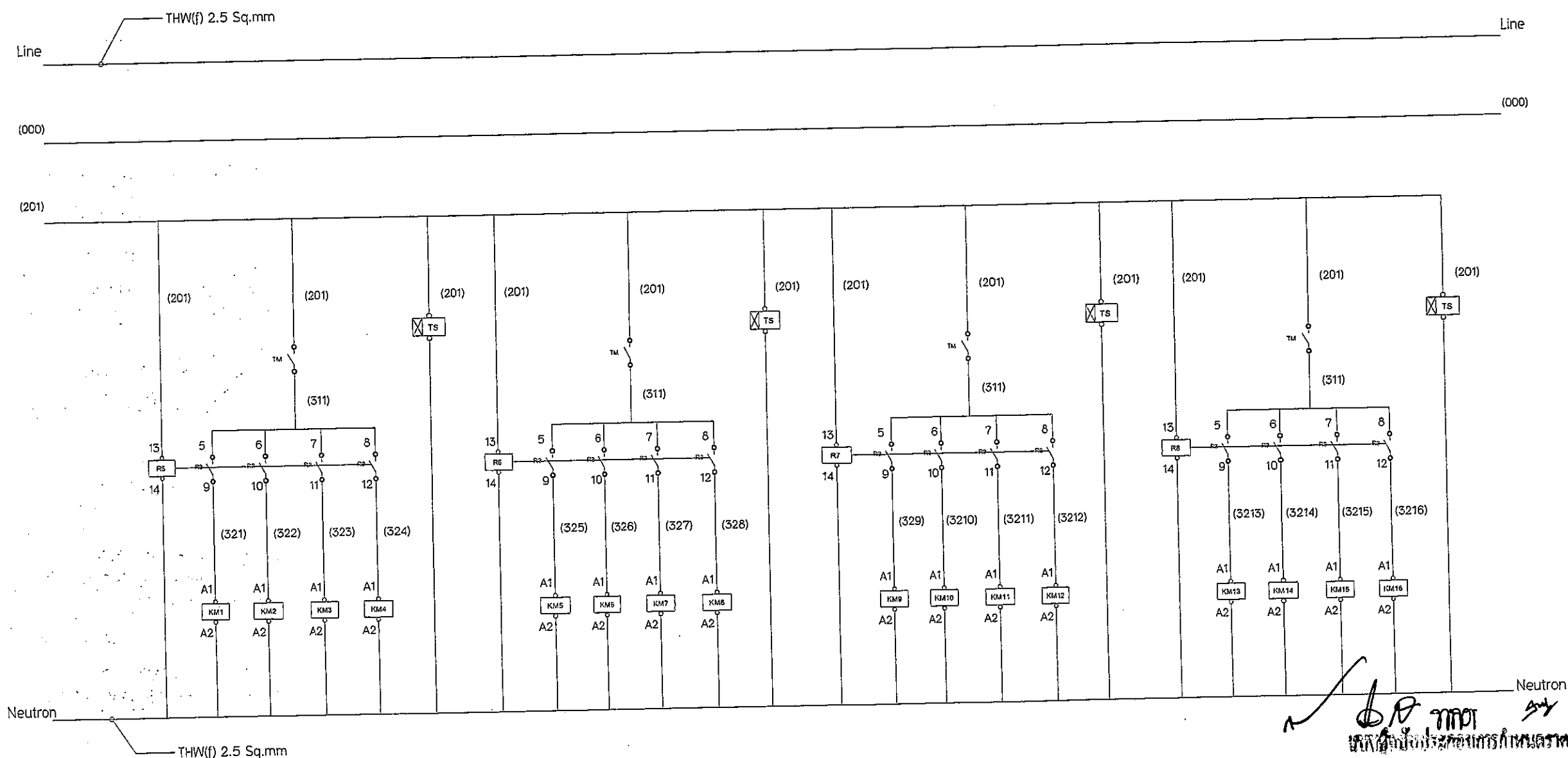
CONTROL DIAGRAM FOR LIGHTING CONTROL (SDP)-Auto(Timer)
