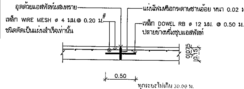
EXPANSION JOINT
