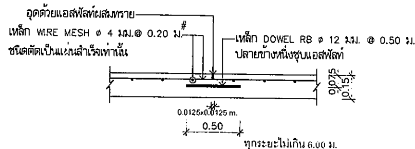
CONTRACTION JOINT
