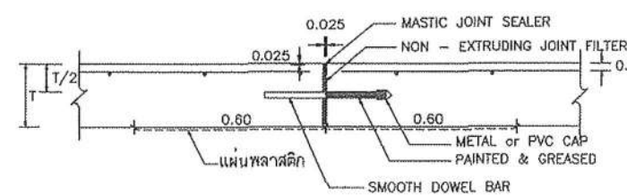
EXPANSION JOINT
