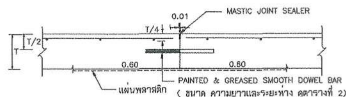
CONSTRUCTION JOINT
