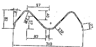
GUARD RAIL
