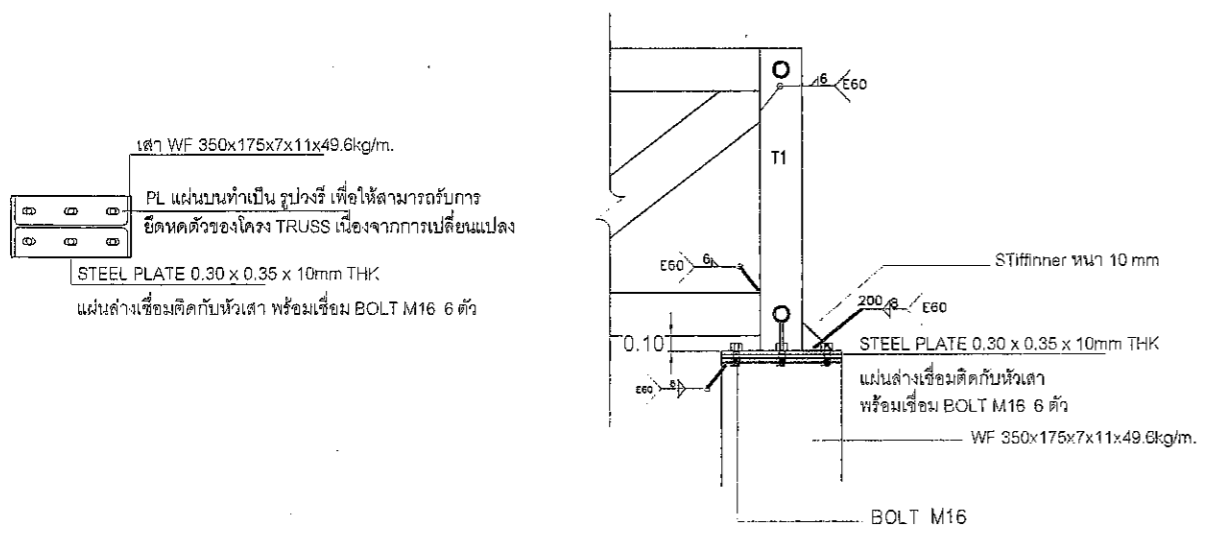
DETAIL FREE SUPPORT
