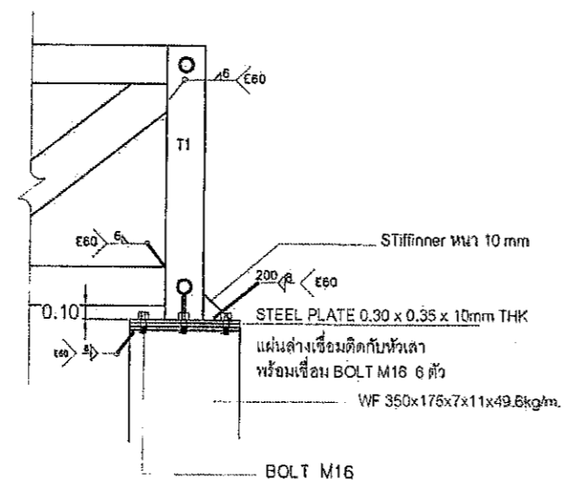
DETAIL FREE SUPPORT
